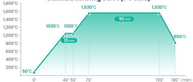
Standard Sintering Curve (1-3 Units)
