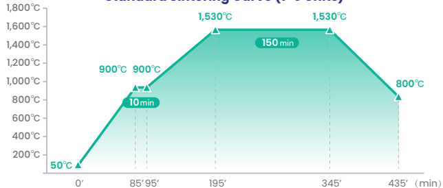
Standard Sintering Curve (1-5 Units)
